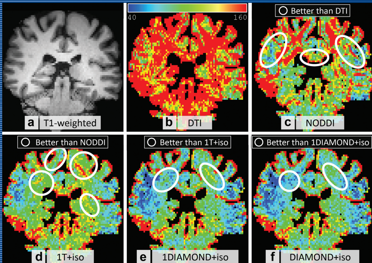
Comparison of five diffusion models with in vivo data by assessment of their generalization error, from the article by Scherrer et al. (pp. 963-977).
